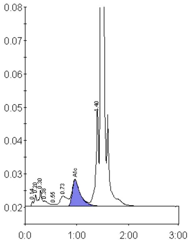
Peak table - ID: 10607200
