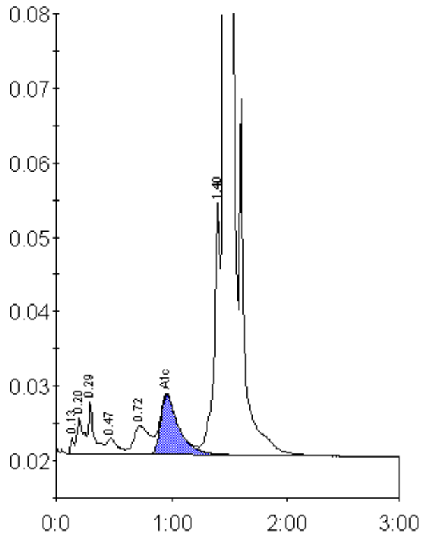
Peak table - ID: 10530551
