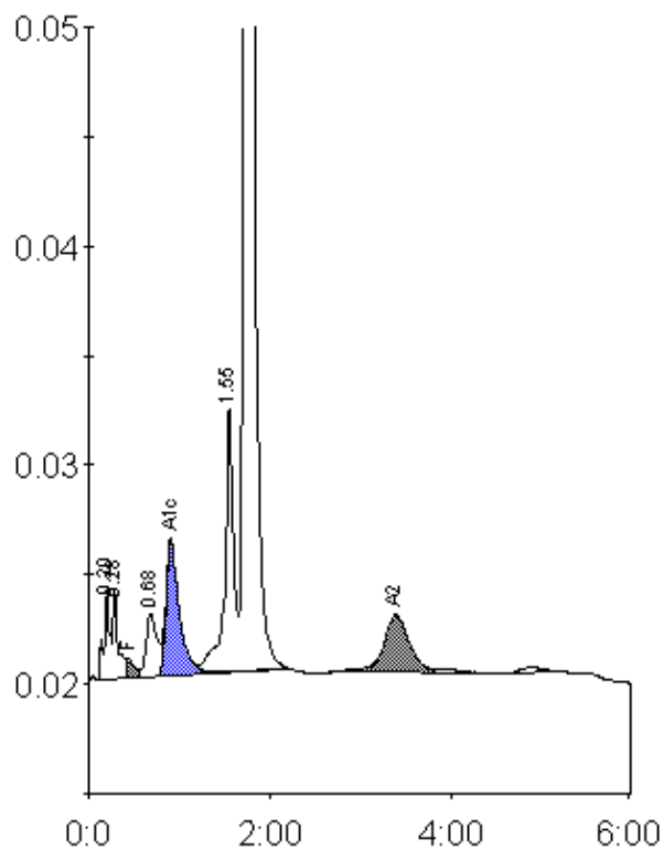
Peak table - ID: 10528883
