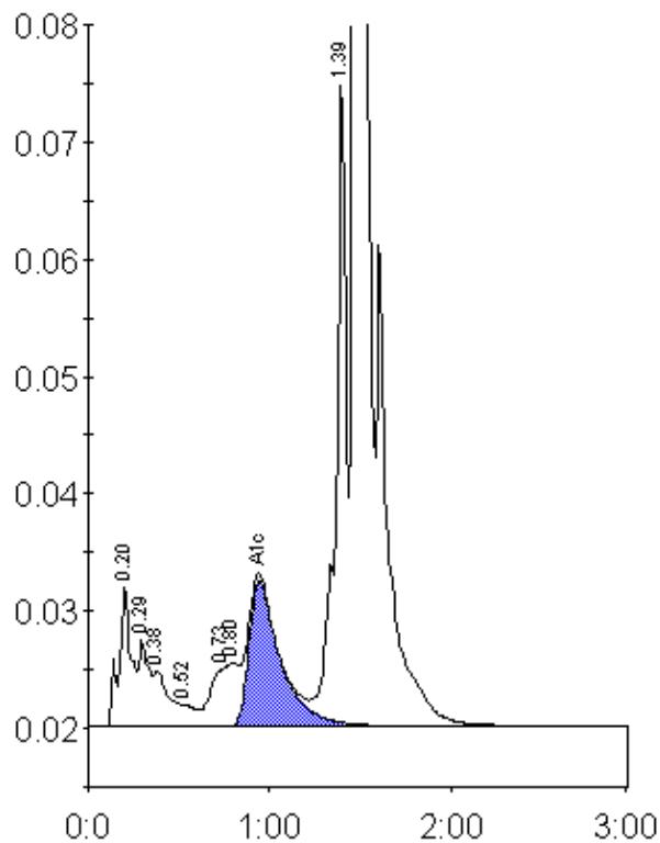
Peak table - ID: 10612198
