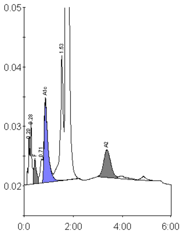
Peak table - ID: 10364362
