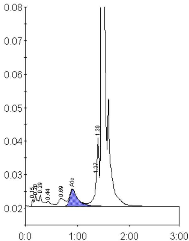
Peak table - ID: 10588897
