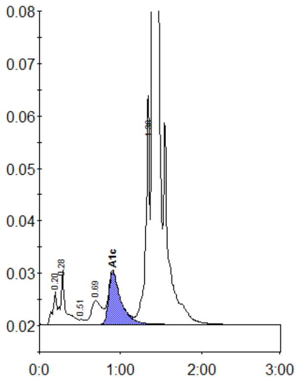
Peak table - ID: 80178396
