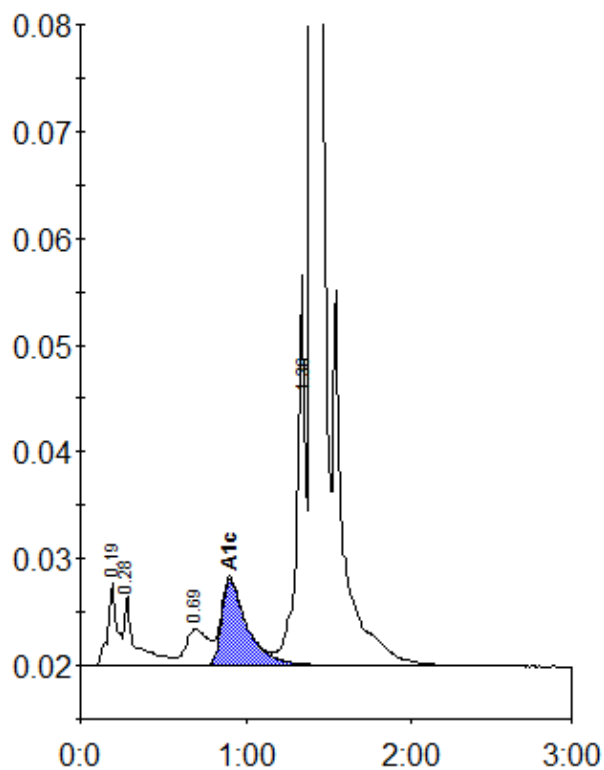
Peak table - ID: 10567481
