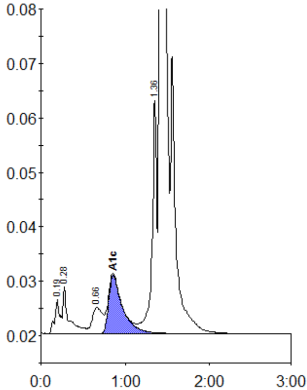
Peak table - ID: 10554359
