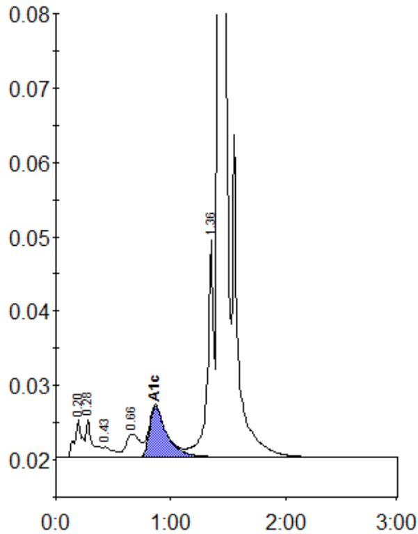
Peak table - ID: 10521034
