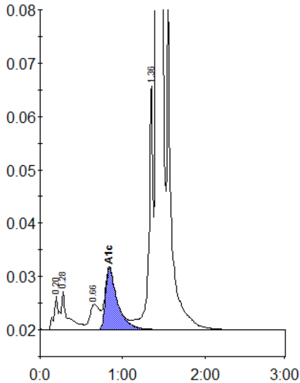
Peak table - ID: 10425792
