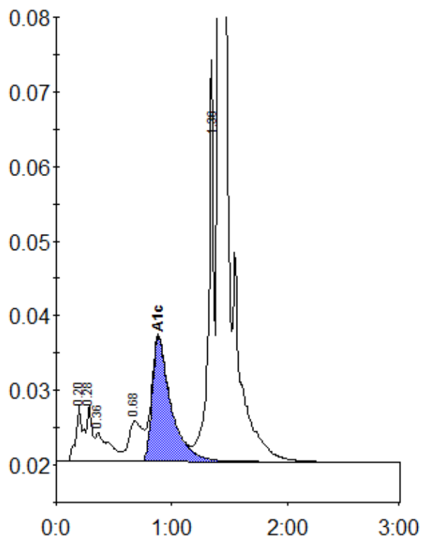
Peak table - ID: 10500557
