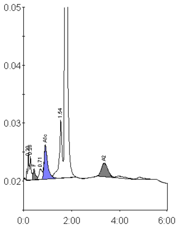
Peak table - ID: 10545008
