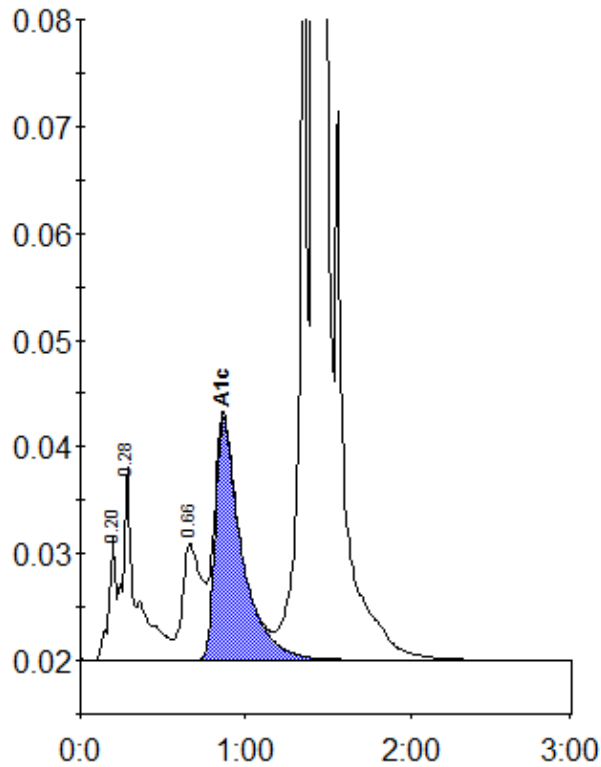
Peak table - ID: 10559212
