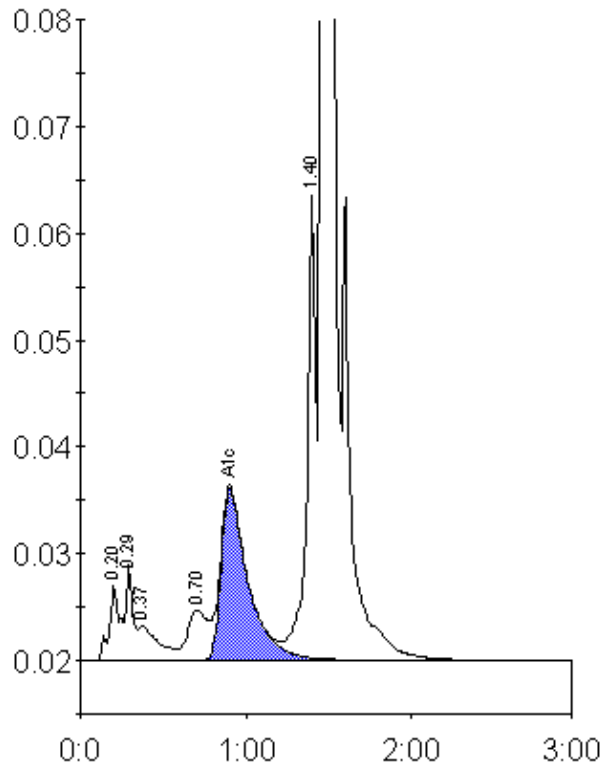
Peak table - ID: 10574610
