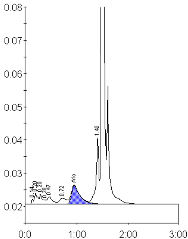
Peak table - ID: 10573567
