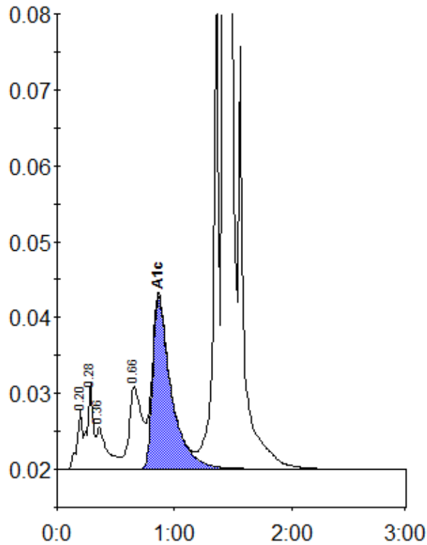
Peak table - ID: 10611602
