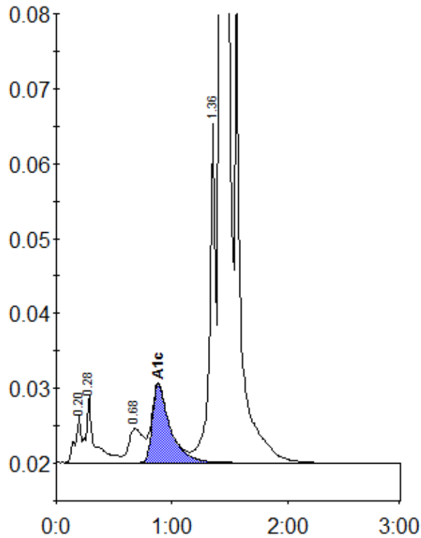
Peak table - ID: 10552465
