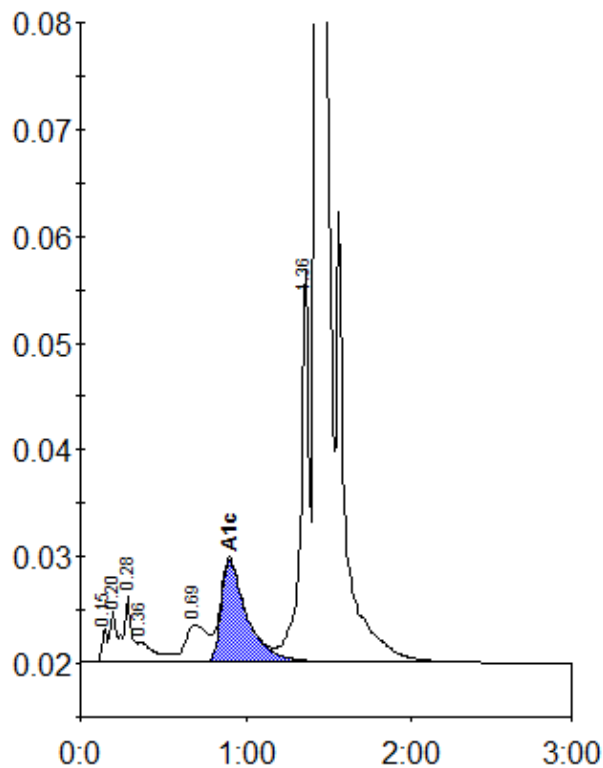
Peak table - ID: 10553931
