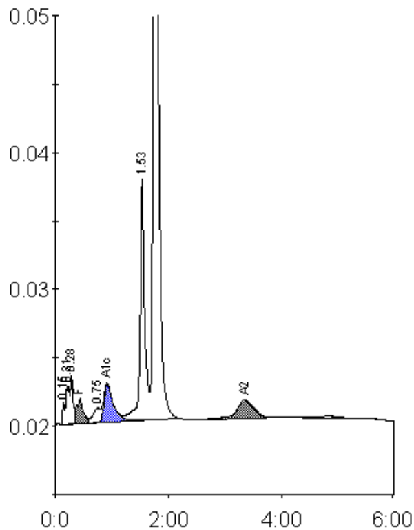
Peak table - ID: S0040035
