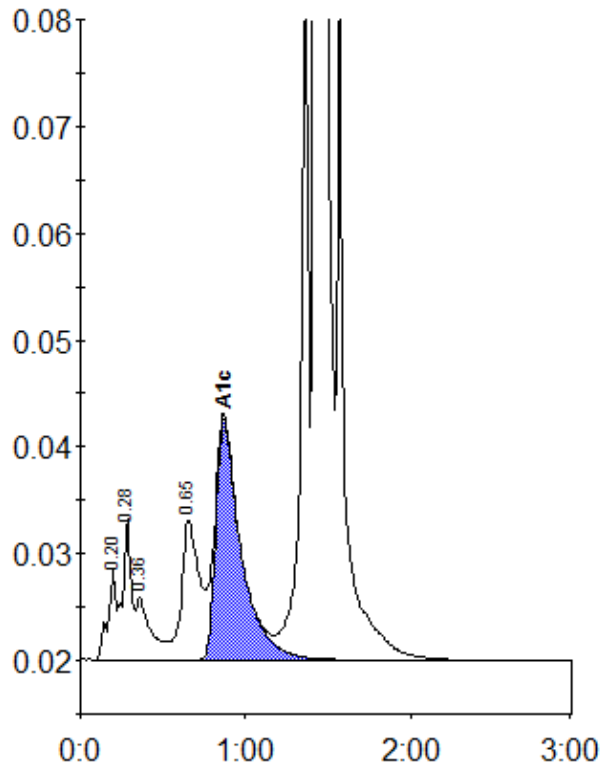
Peak table - ID: 10468326
