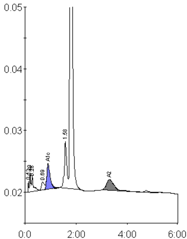
Peak table - ID: 10566691
