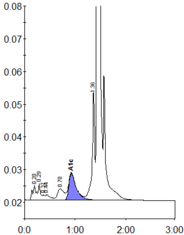
Peak table - ID: 10618486
