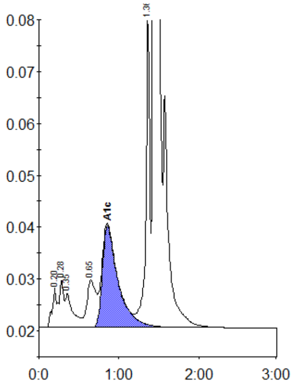
Peak table - ID: 10378231
