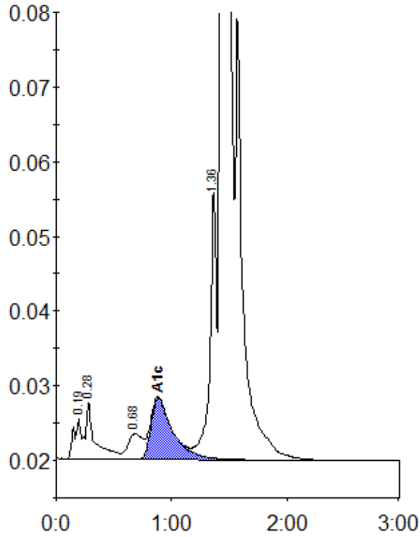
Peak table - ID: 10571850
