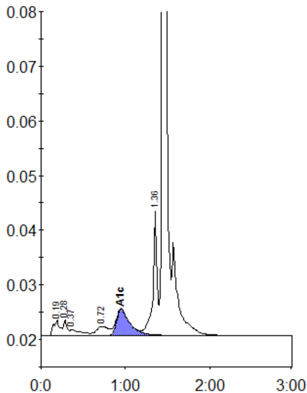
Peak table - ID: 10630399
