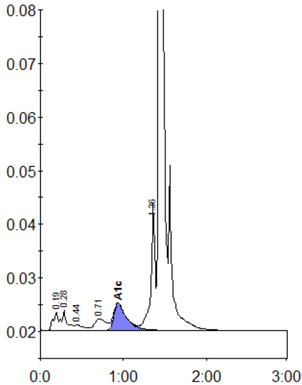
Peak table - ID: 10468409
