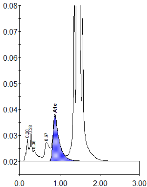
Peak table - ID: 10618337
