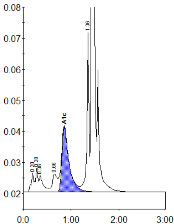
Peak table - ID: 10633436
