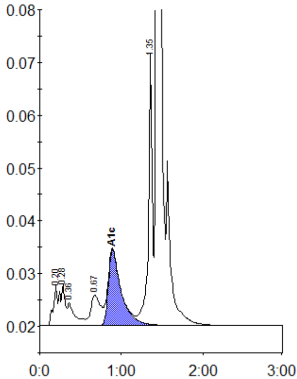
Peak table - ID: 10630661
