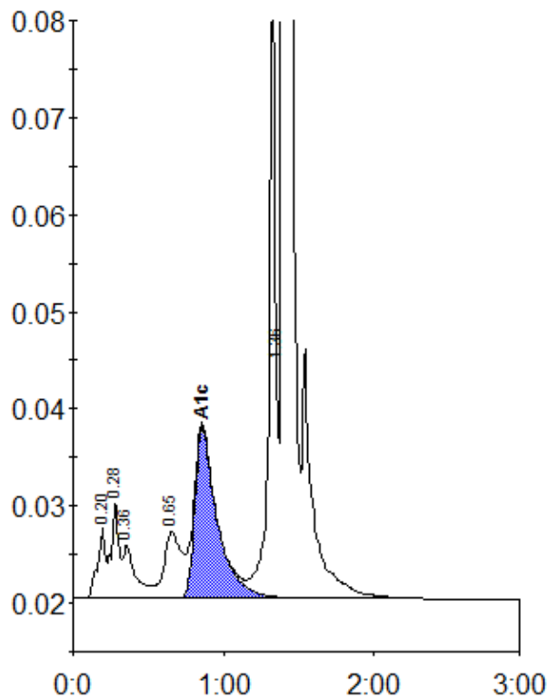
Peak table - ID: 10630466
