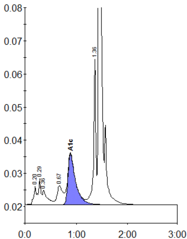
Peak table - ID: 10440145
