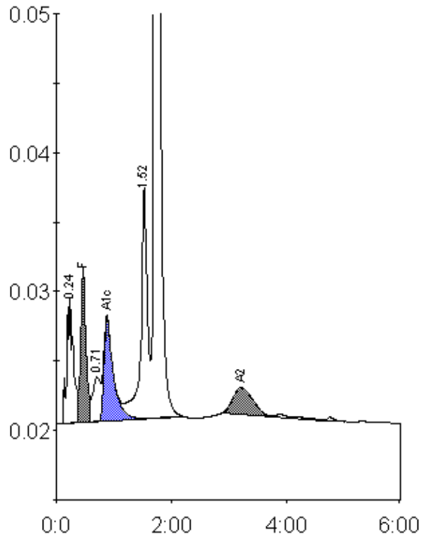
Peak table - ID: 10435675
