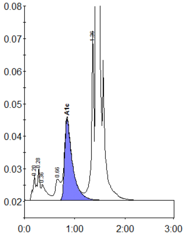
Peak table - ID: 10450757
