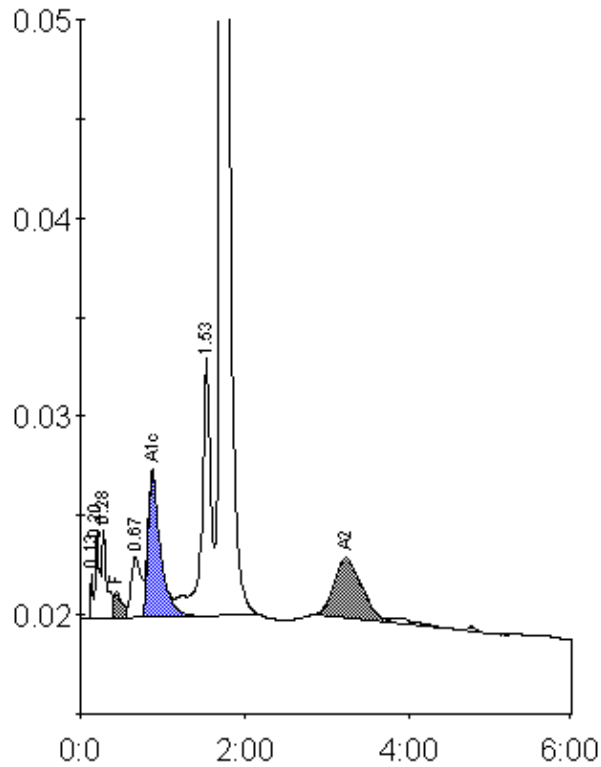
Peak table - ID: 10219116
