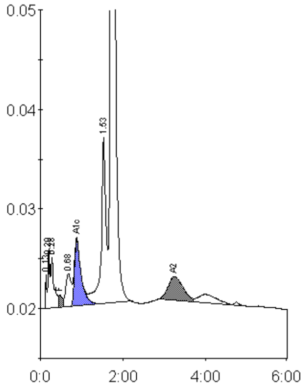
Peak table - ID: 10437317
