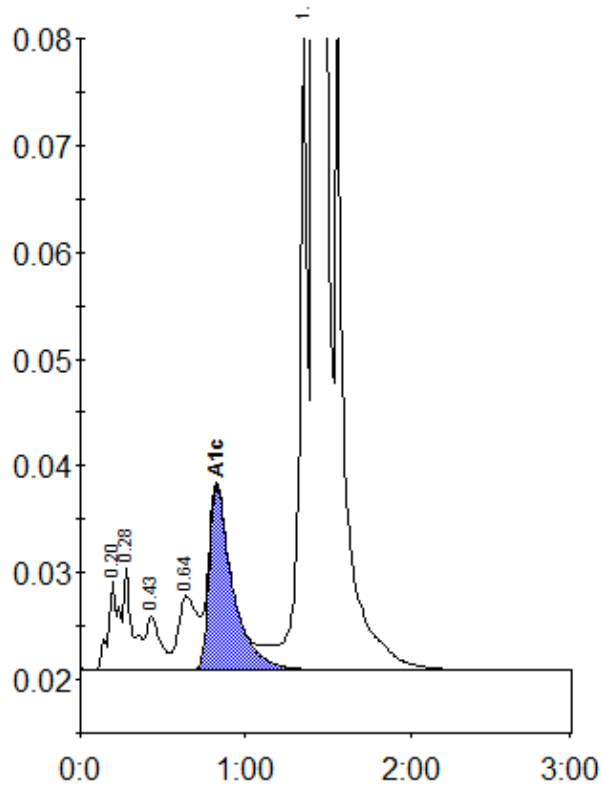
Peak table - ID: 10431736
