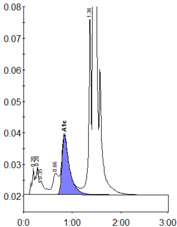
Peak table - ID: 10355506
