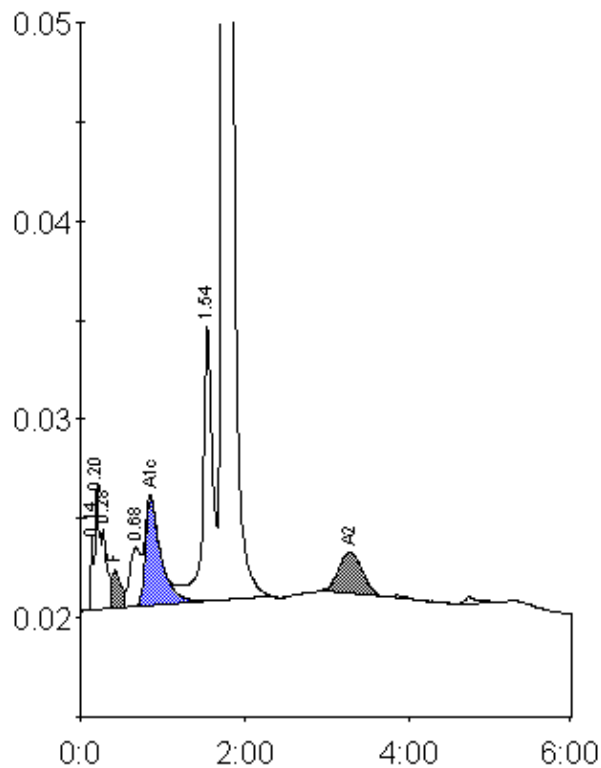
Peak table - ID: 10408988
