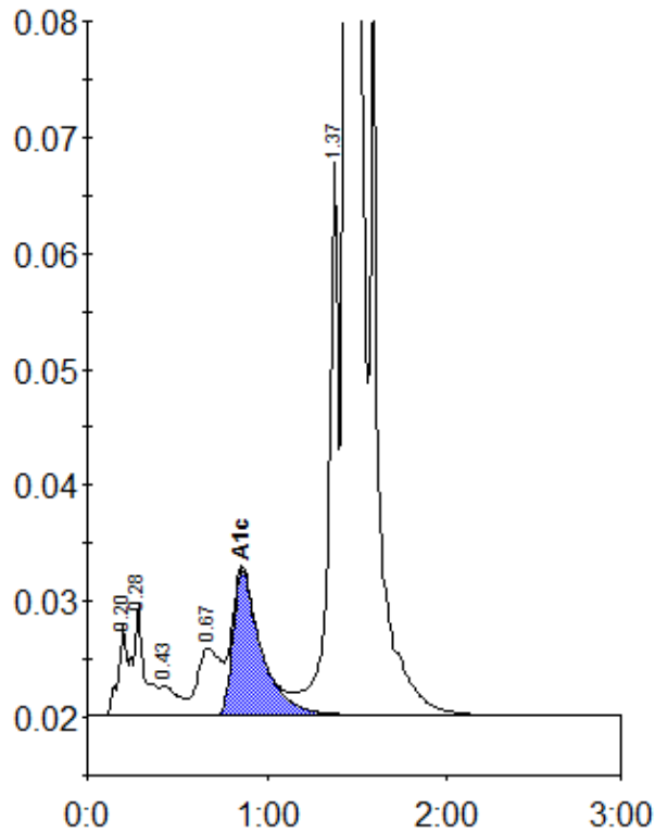
Peak table - ID: 10406578
