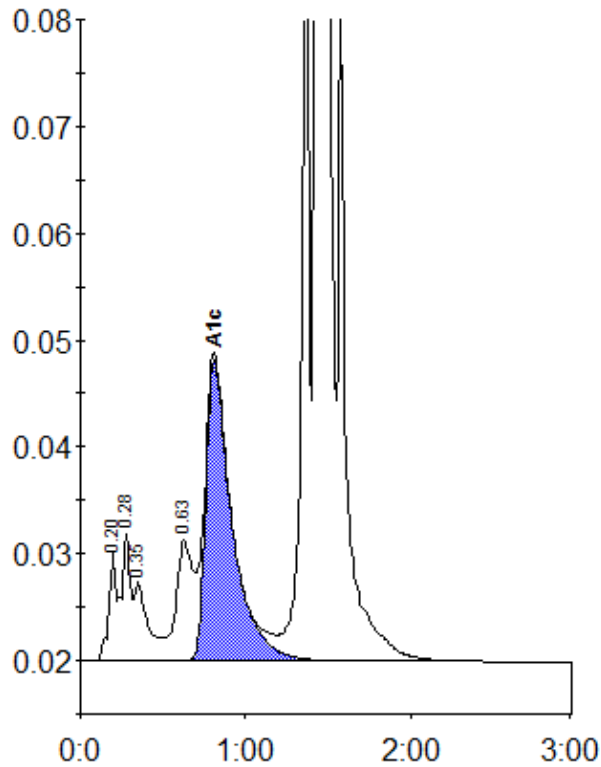
Peak table - ID: 10421927
