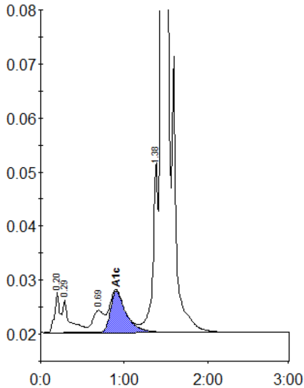
Peak table - ID: 10408820
