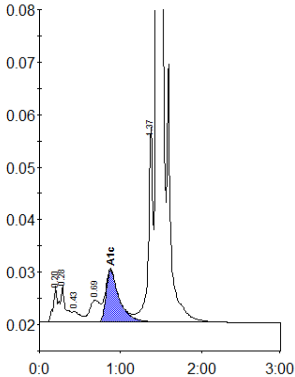
Peak table - ID: 10365030
