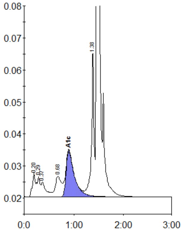
Peak table - ID: 10337910
