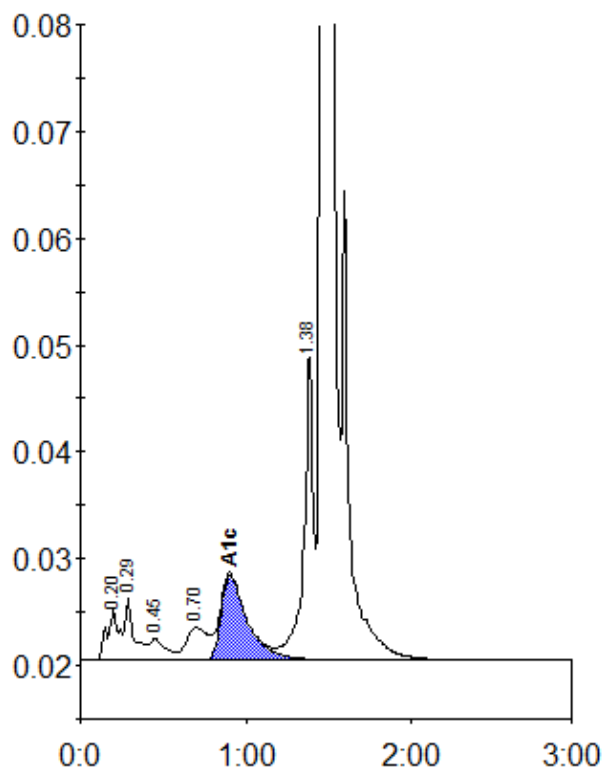
Peak table - ID: 10316493
