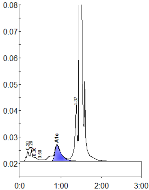
Peak table - ID: 10387234
