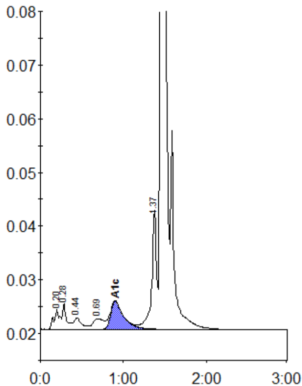
Peak table - ID: 10312125
