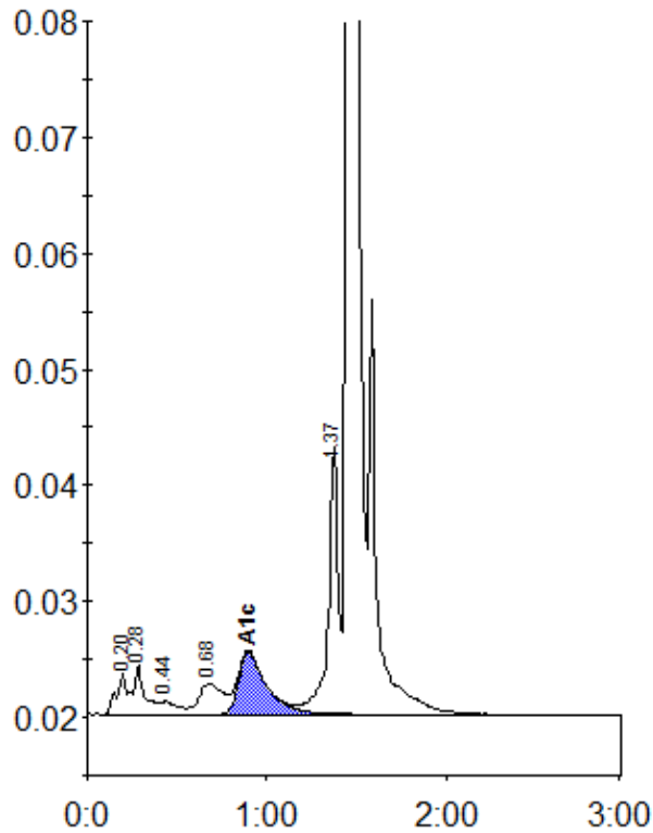
Peak table - ID: 10391098
