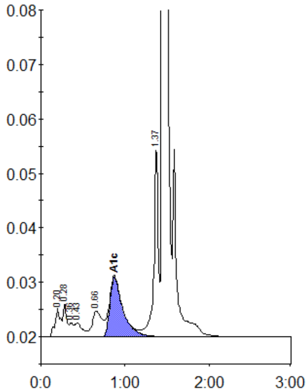
Peak table - ID: 10387057
