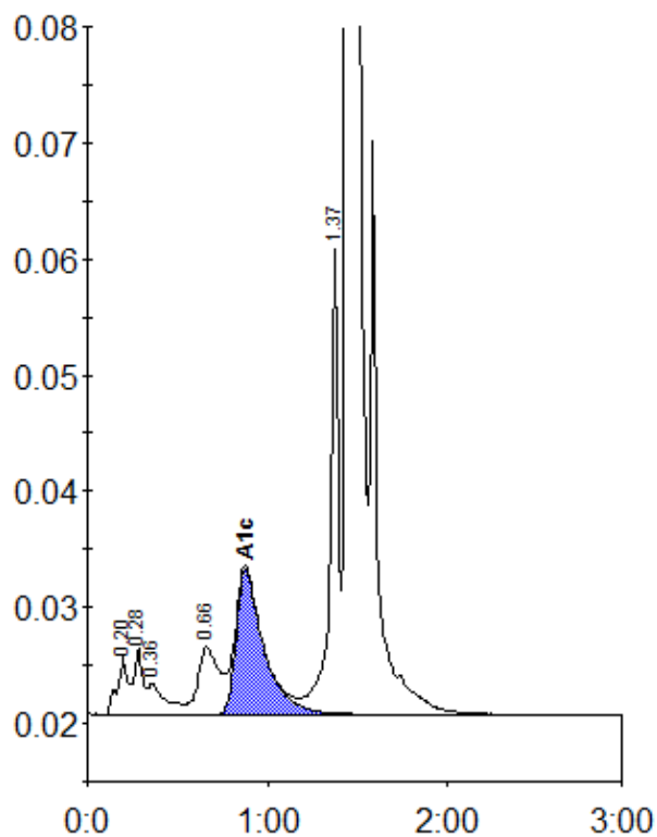
Peak table - ID: 10391922
